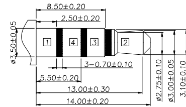
MATE PLUG (4 POLE)
