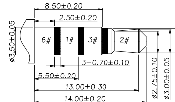
MATE PLUG (4 POLE)
