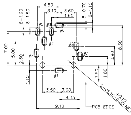
RECOMMENDED P.C.B LAYOUT TOP VIEW (TOLRANCE:±0.05)
